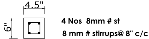
LINTEL OVER 4.5" WALL
