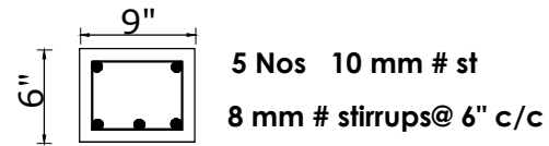
LINTEL OVER 9" WALL
