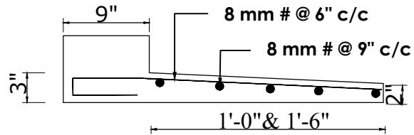
SUNSHADE DETAILS
