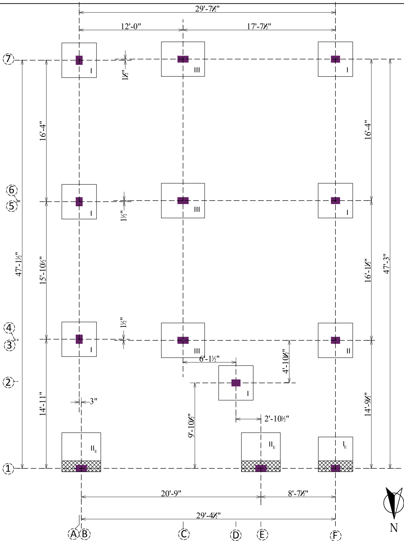
CENTRE LINE LAYOUT-REVISED
